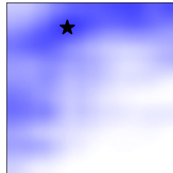
Deterministic prediction
